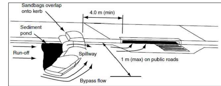
SANDBAG SEDIMENT COLLECTION DAM REFER IECA STD. DWG. OG-01 FOR DETAILS.
