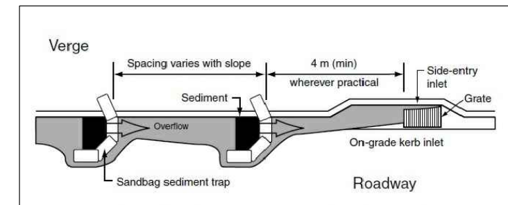
TYPICAL LAYOUT ON-GRADE KERB SEDIMENT TRAP REFER IECA STD. DWG. OG-01 FOR DETAILS.
